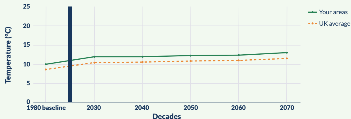
Figure 2 – Cambridgeshire vs UK average temperature increases, Local Climate Adaptation Tool (2024) https://www.lcat.uk/
