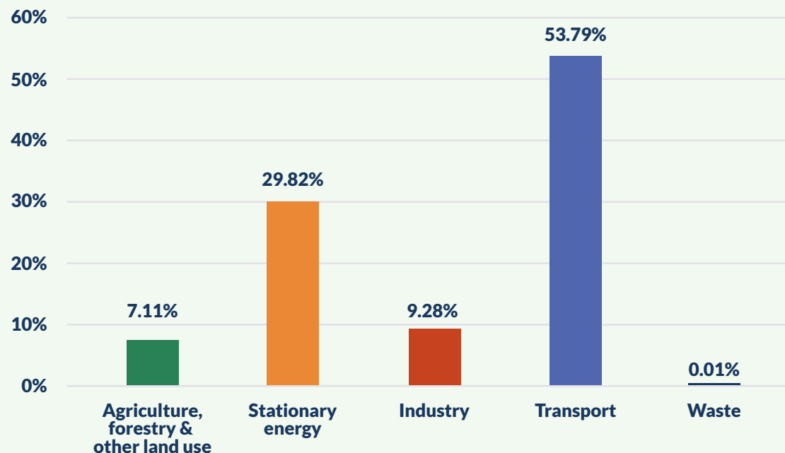
Figure 3 – South Cambridgeshire District Council Carbon Emissions by GHG Sector using 2023 DESNZ emissions data for South Cambridgeshire District Council. Latest available emissions data from DESNEZ as of January 2026
