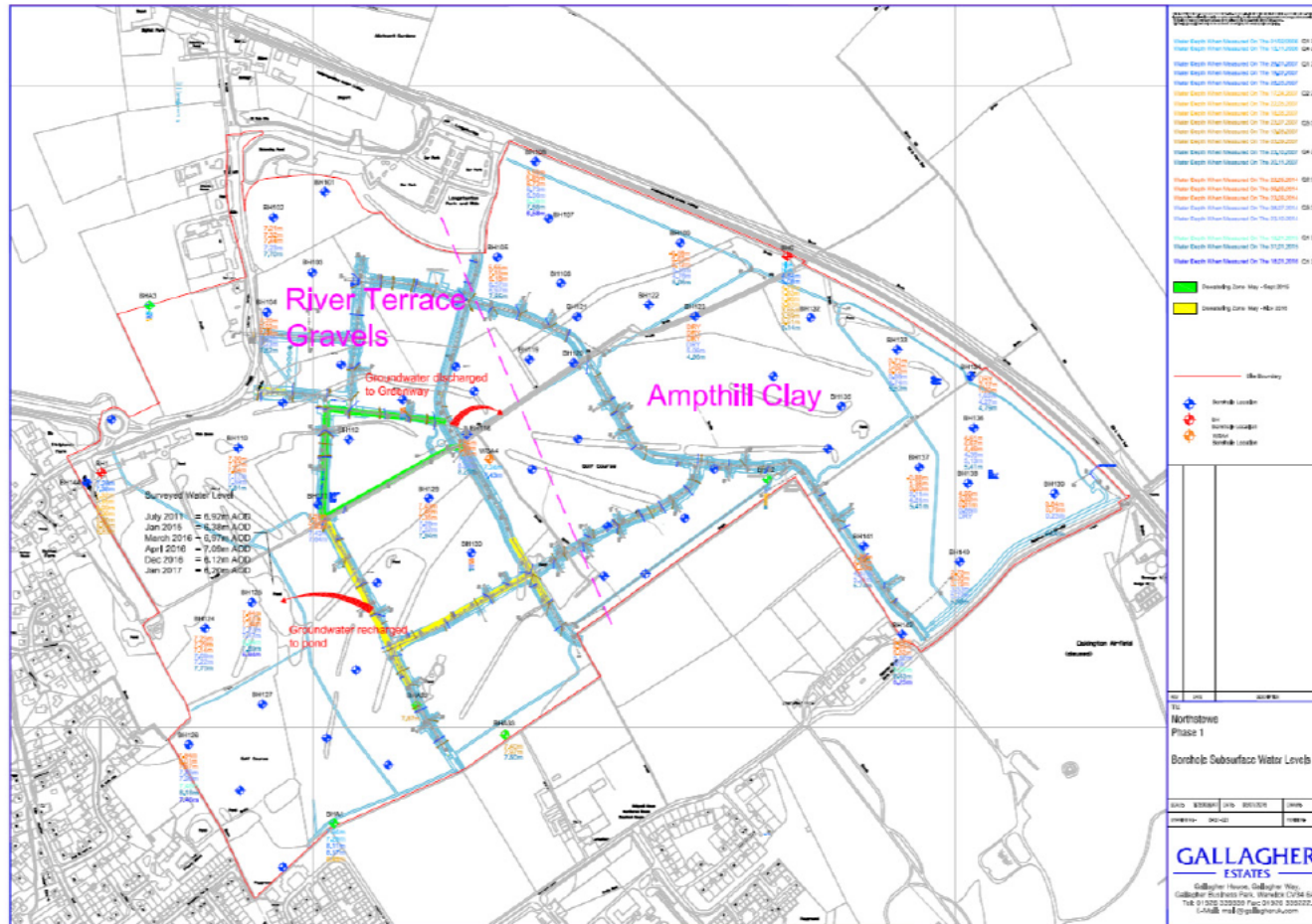
Figure 4.1: Borehole subsurface water levels. Site of Phase 1A dewatering indicated in green. Site of Phase 1B dewatering indicated in yellow
