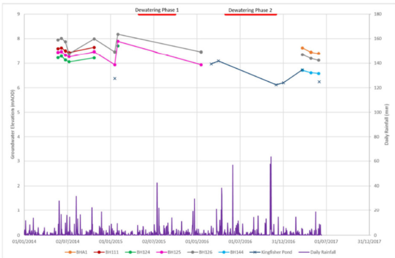
Figure 3.7: Groundwater elevation for Northstowe monitoring boreholes, surface water elevation for the Kingfisher Pond and daily rainfall for the period January 2014 to May 2017
