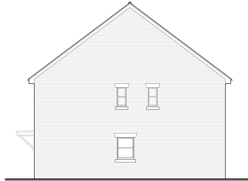
SIDE ELEVATION
