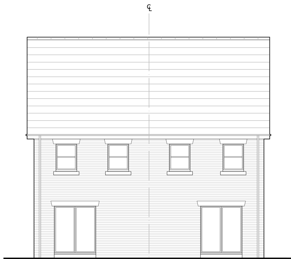
REAR ELEVATION
