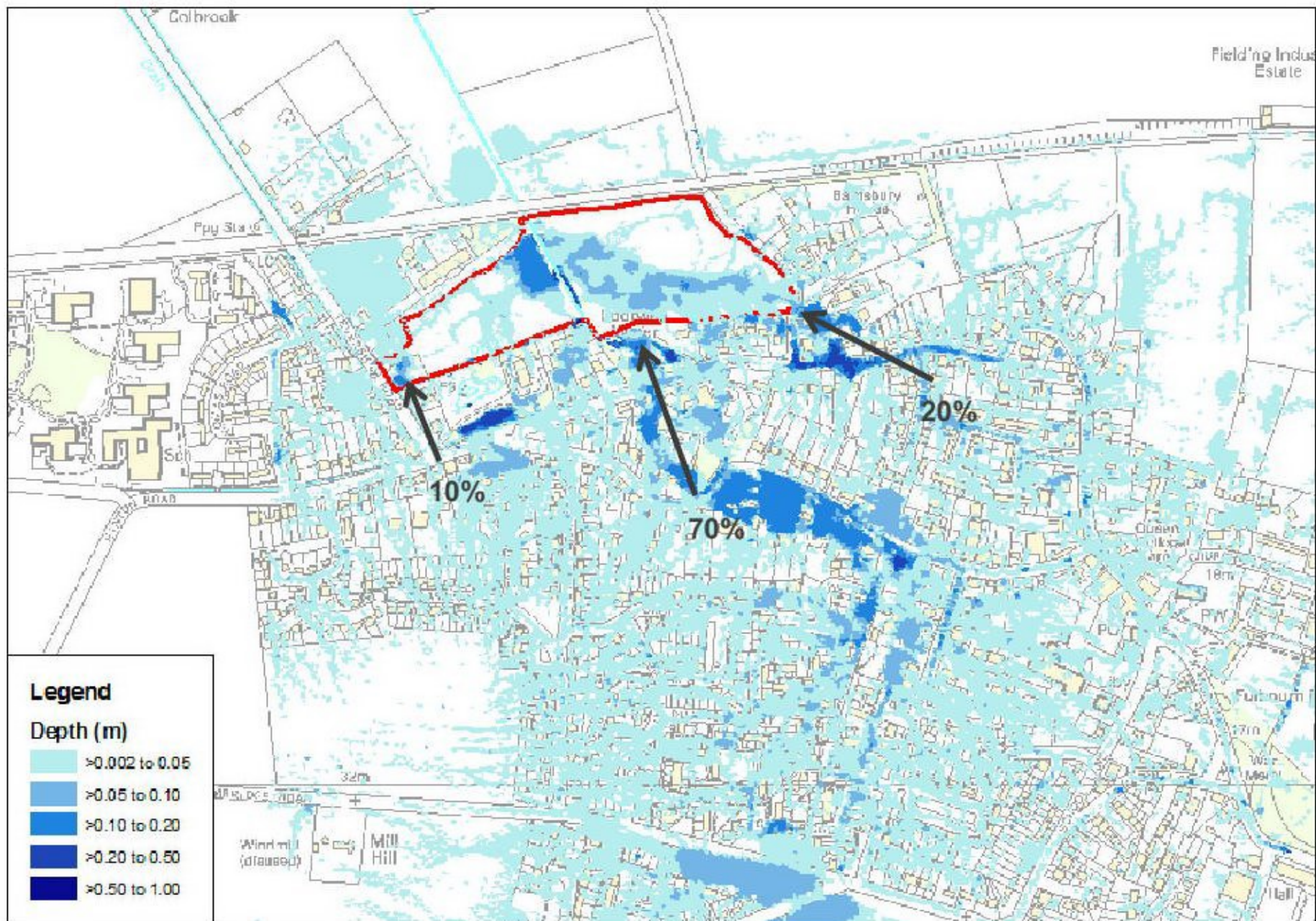
Figure 2.4: Surface water flow paths on the site
