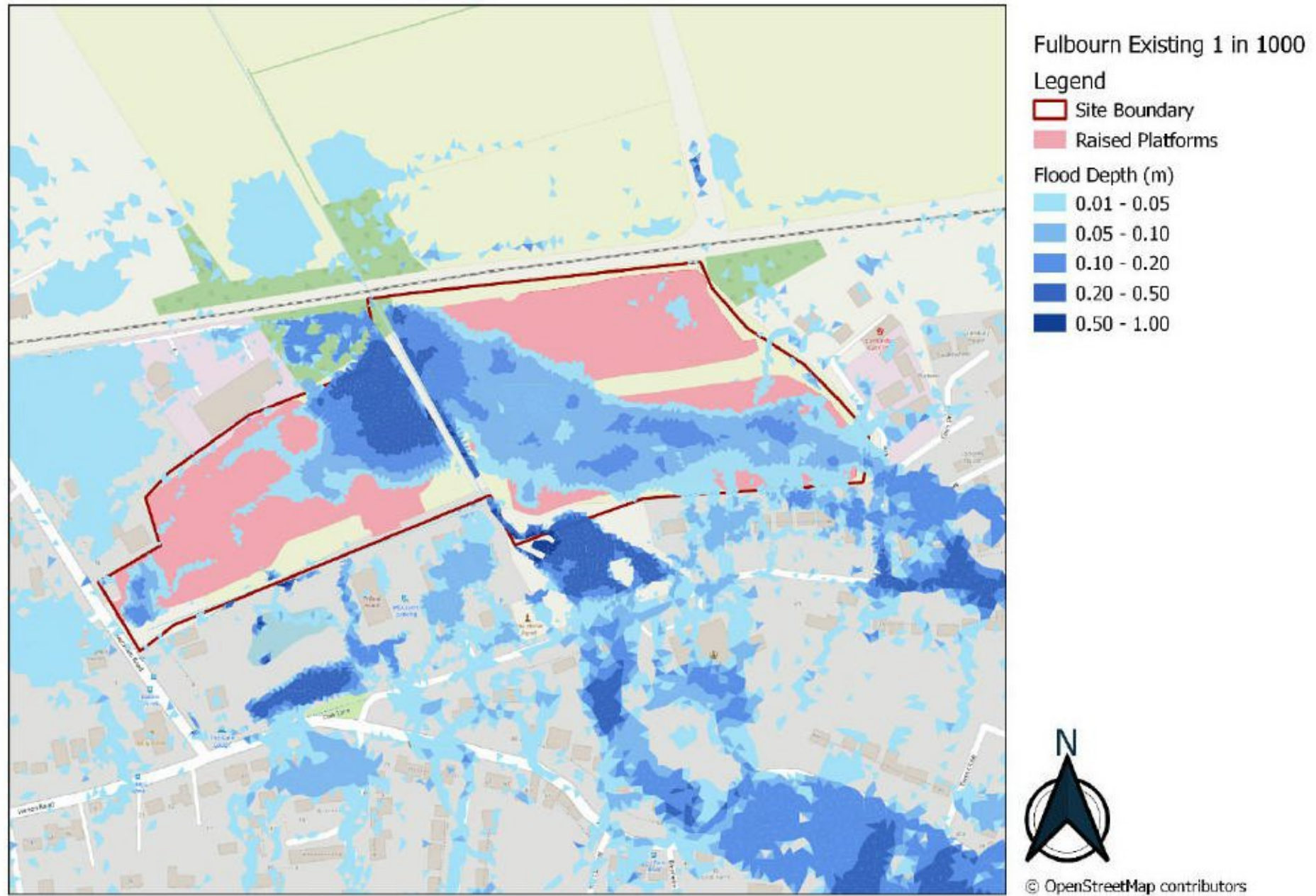
Figure 4.4: Surface water flood depths for the 1 in 1,000 year rainfall
