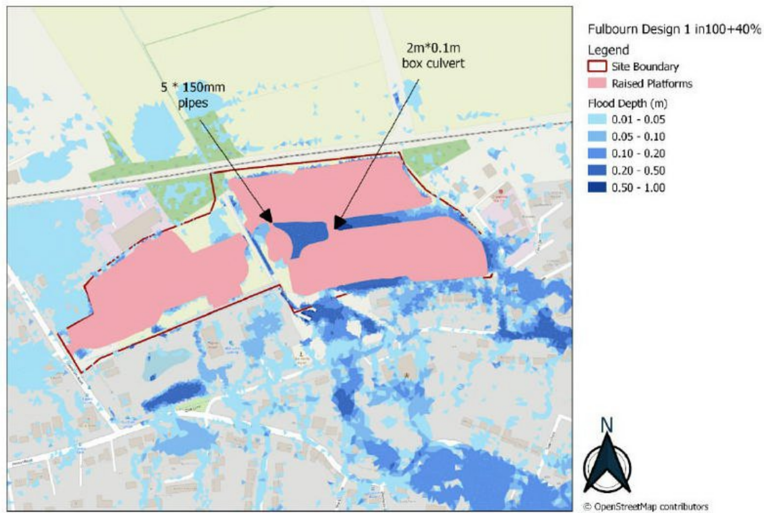
Figure 4.7: Surface water flood depths for the 1 in 100 year climate change rainfall with development in place
