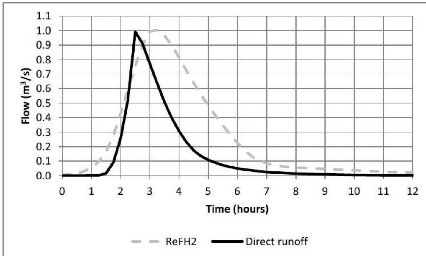
Figure 2.5: Flow hydrographs from ReFH2 and the Direct Rainfall method for the 3.25 hour 100 year storm
