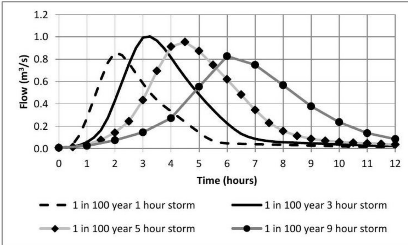
Figure 2.3: ReFH2 flood flow hydrographs
