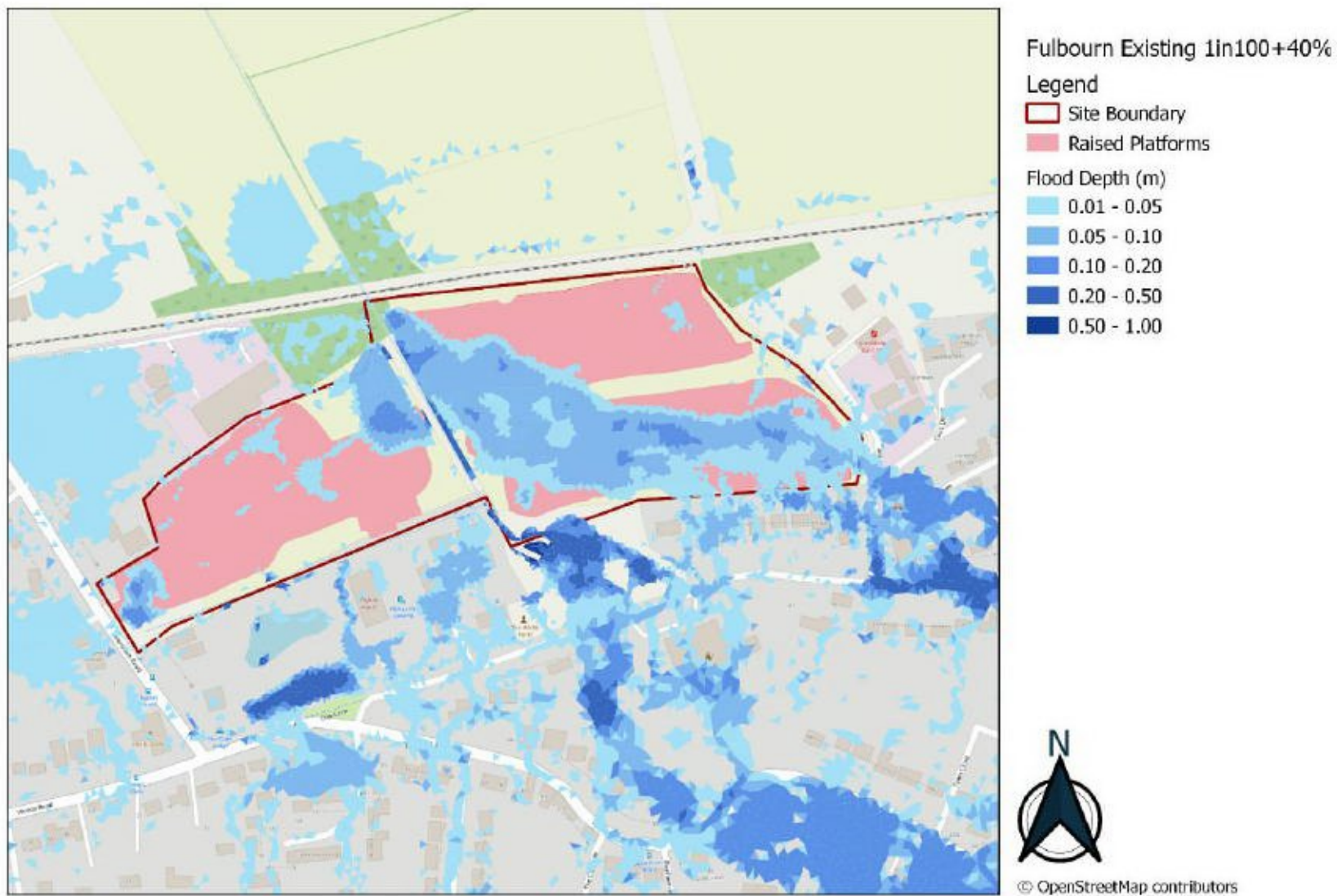
Figure 4.3: Surface water flood depths for the 1 in 100 year rainfall plus 40% climate change
