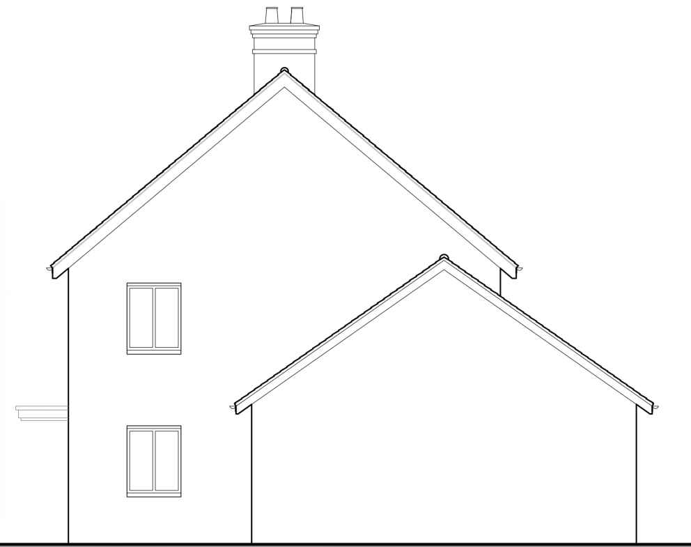
SIDE ELEVATION 1
